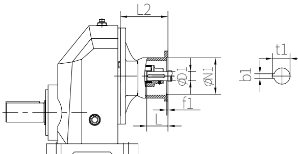
6.2 C series dimensions of AS input flange
